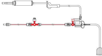
BP-S00028 Single transducer set with self-flushable needle free valve
