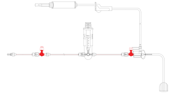
BP-S00031 Single transducer closed blood sampling set
